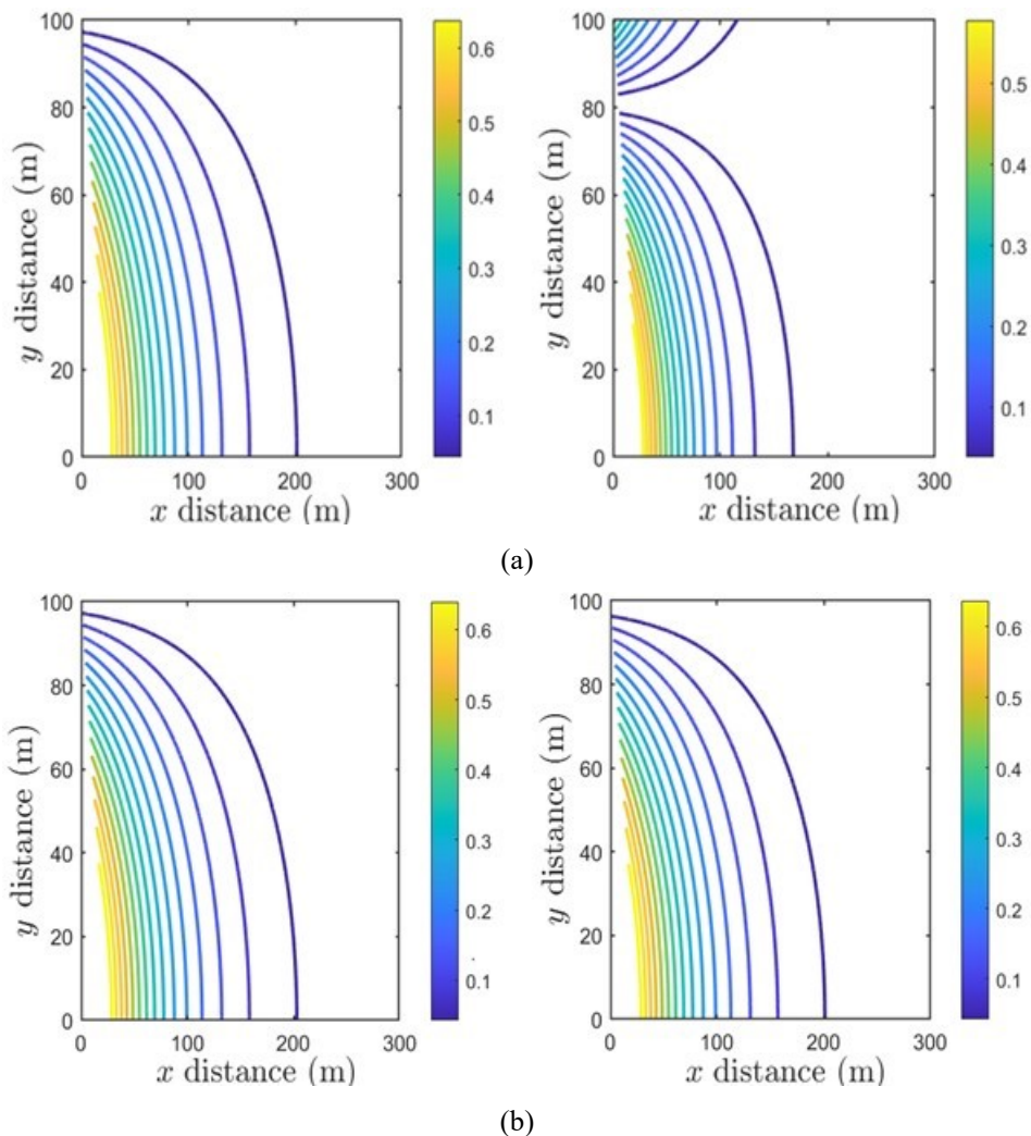
Figure 4: Shape of the normalized hydrodynamic pressure curves for c=1 , \theta=15^\circ , and \zeta=1\% : (a) Low excitation frequency, \omega=0.49 rad/s, (b) High excitation frequency, \omega=3.13 rad/s; left: without surface-wave effect, right: with surface-wave effect
