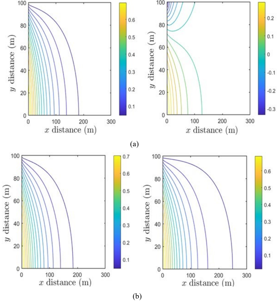
Figure 3: Shape of the normalized hydrodynamic pressure curves for c=0 , \theta=0^\circ , and \xi=1\% : (a) Low excitation frequency, \omega=0.49 rad/s; (b) High excitation frequency, \omega=3.13 rad/s; left: without surface-wave effect, right: with surface-wave effect
