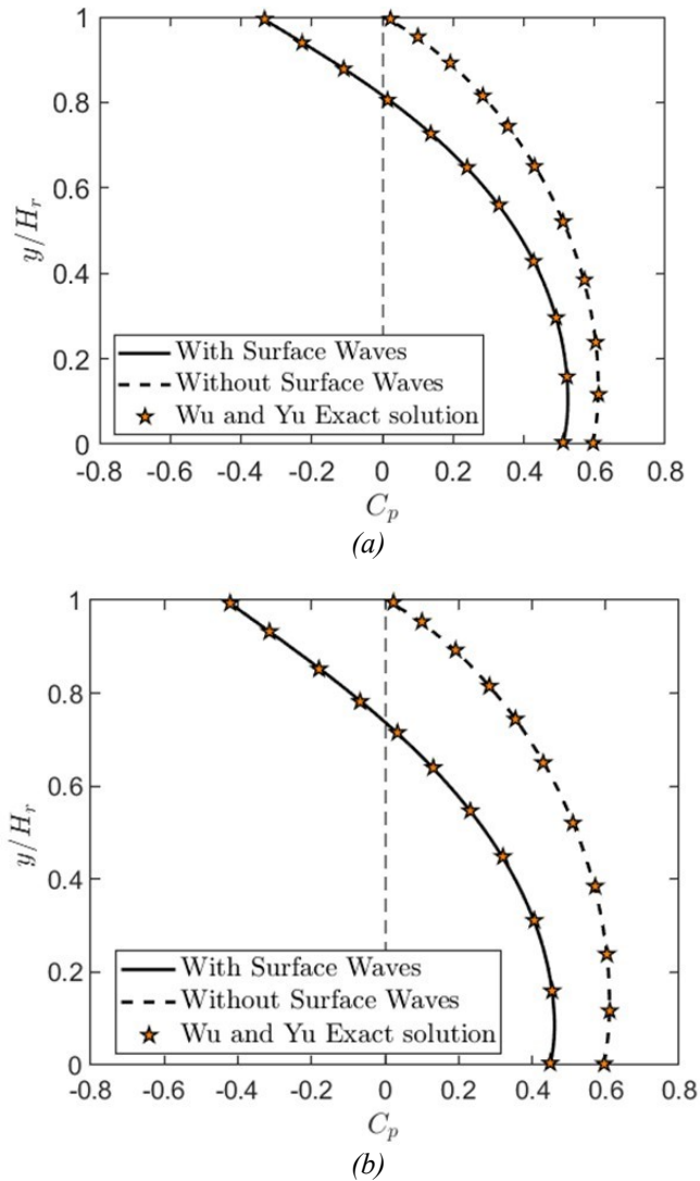
Figure 2: Convergence of the present solution toward the Wu and Yu (1989) exact solution for c = 1, \theta = 15^\circ : (a) Case of CW = 0.2 , (b) Case of CW = 0.3
