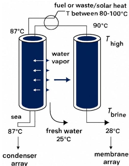
Figure 2: Integrated design of Memstill technology.
