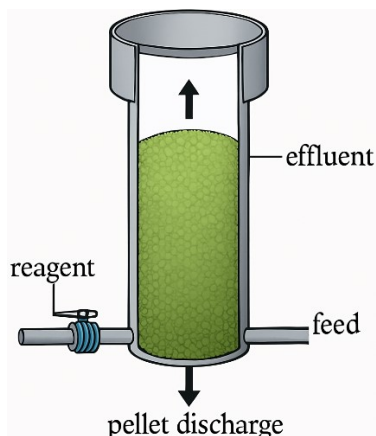
Figure 1 Crystalactor (Giesen, 1999).
